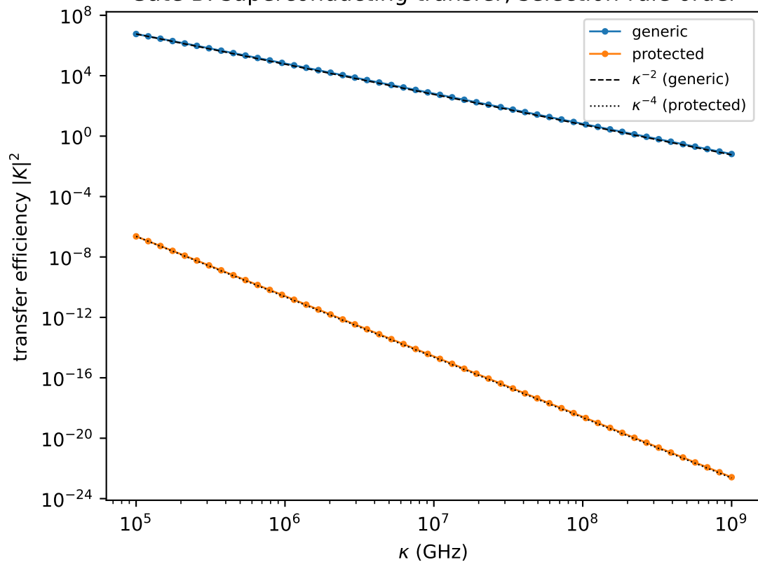
Gate B: superconducting transfer, selection-rule order
